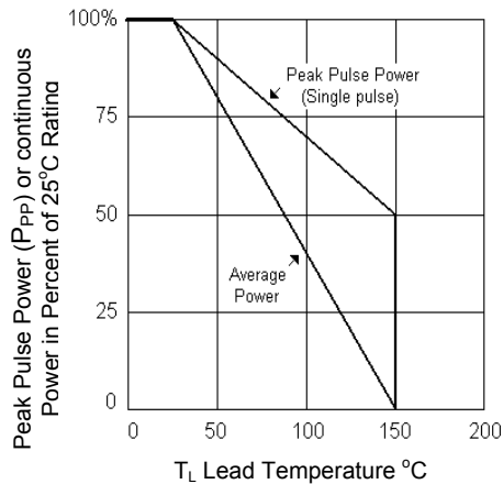
FIGURE 3 - Derating Curve
