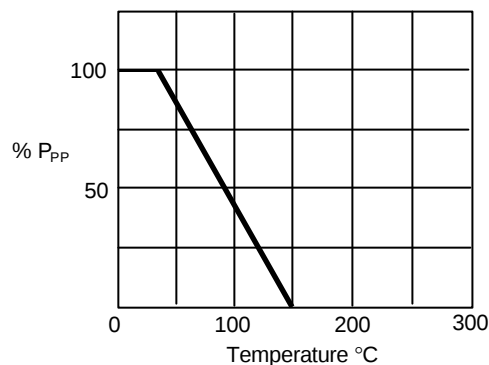
Figure 4 - Derating Curve
