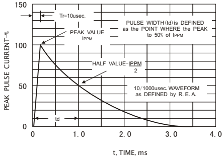
FIG. 3-PULSE WAVEFORM
