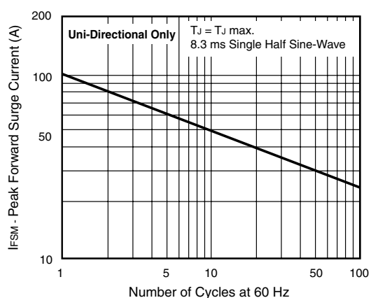
Figure 6. Maximum Non-Repetitive Forward Surge Current
