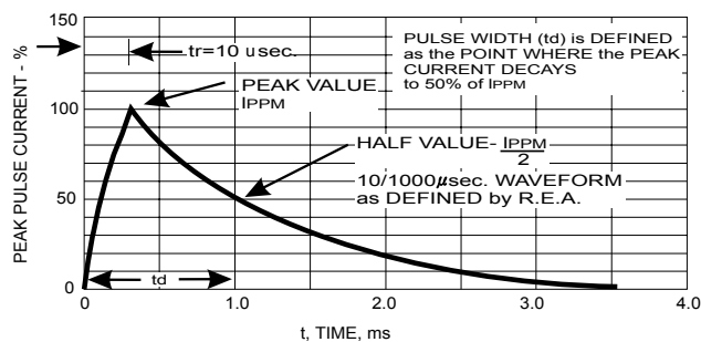
FIG.3- PULSE WAVEFORM
