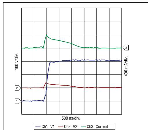
P500-G Solution: 5000 V Lightning 2/10 µsec, 500 A
