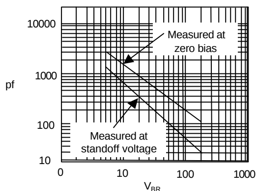
Figure 3 - Typical Capacitance
