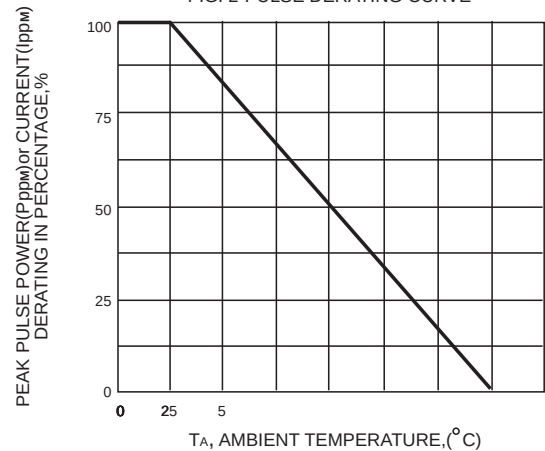
FIG. 2-PULSE DERATING CURVE
