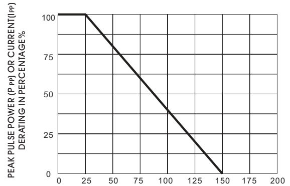
FIGURE 2-PULSE DERATING CURVE
