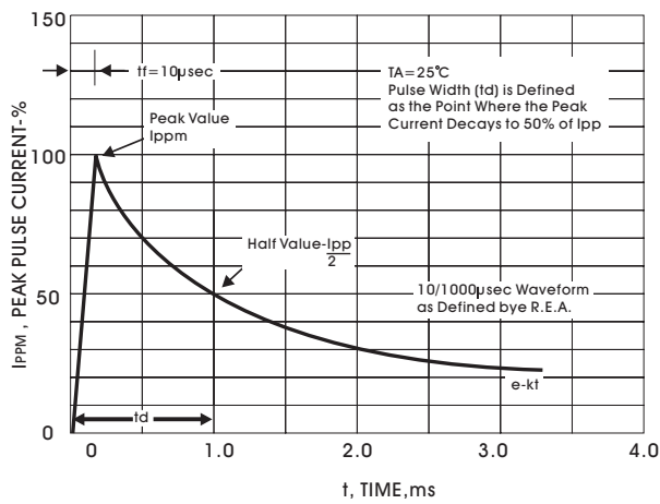
FIGURE 3-PULSE WAVEFORM
