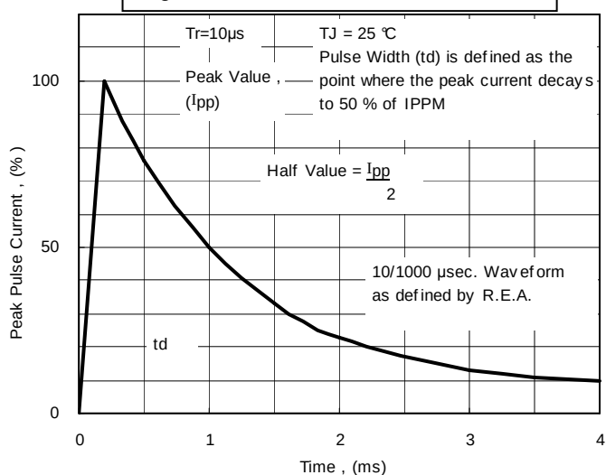
Fig. 5 - Pulse Pulse Waveform
