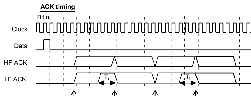
Figure 5: ACK timing diagram
