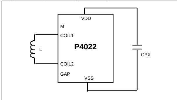
Figure 1: Low frequency inductive transponder implementation.
