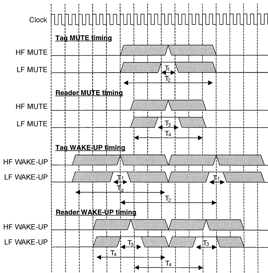
Figure 6: MUTE and WAKE-UP timing diagrams
