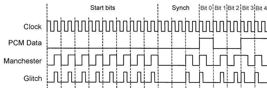
Figure 7: Data encoding methods
