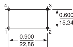
Recommended Board Layout
