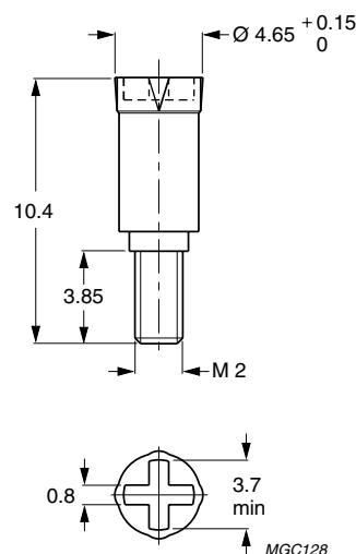
Fig.2 P22/13 inductance adjuster.
