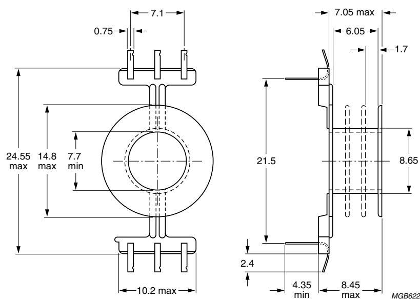
Fig.4 P18/11 coil former for PCB mounting; 6-pins.
