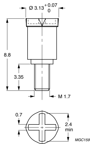
Fig.2 P18/11 inductance adjuster.
