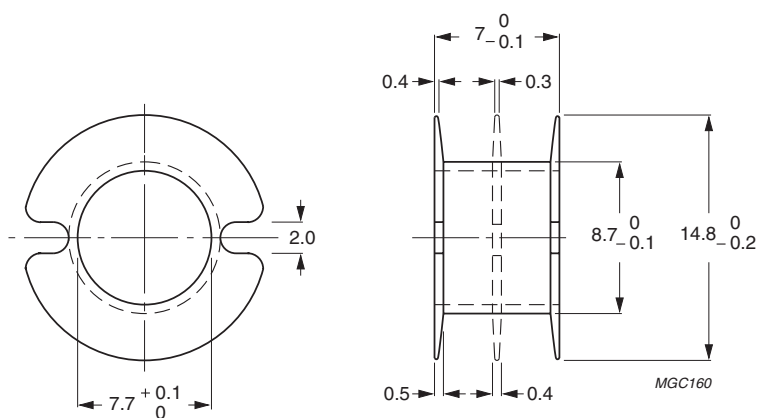
Fig.3 CP-P18/11 coil former.
