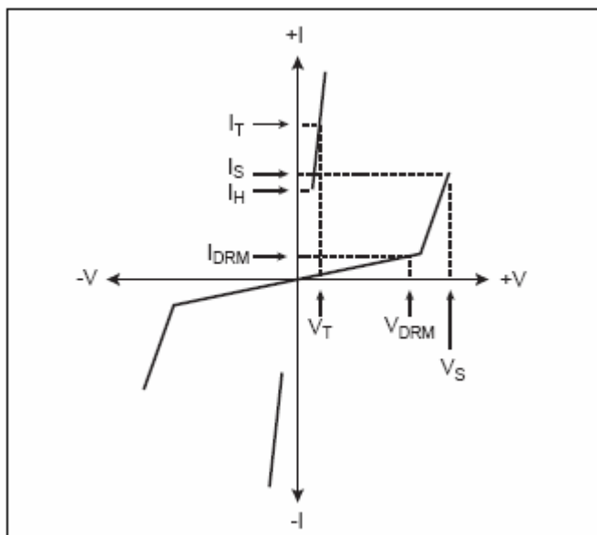
Figure1 V-I Characteristics
