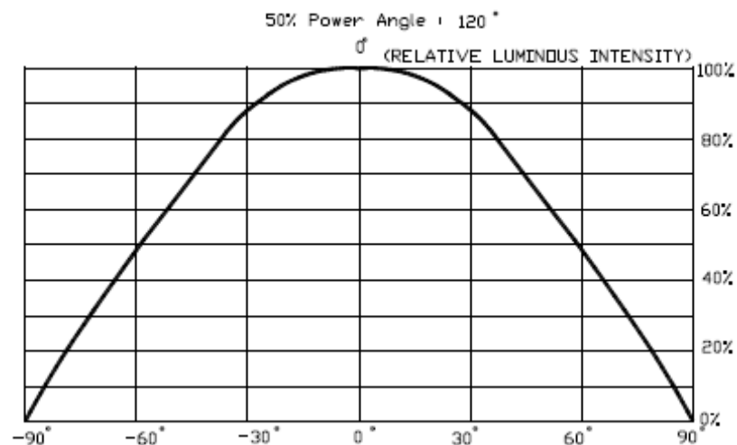
Far Field Pattern
