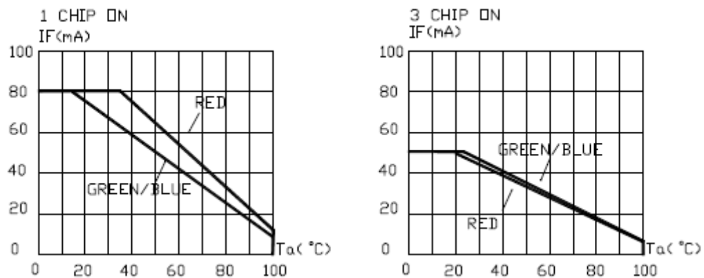
Maximum Forward DC Current vs Ambient Temperature
