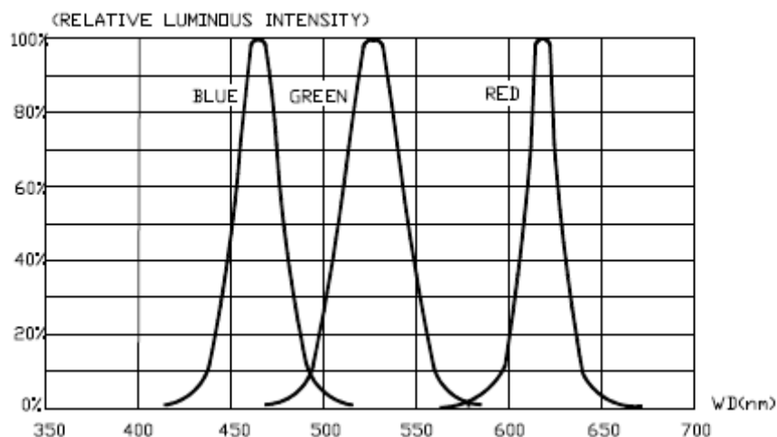
Relative Intensity vs Dominant Wavelength
