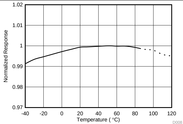
Figure 8. Full-Scale-Range Matching (Highest 6 Ranges)
