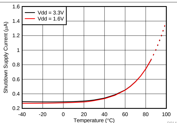
Figure 21. Shutdown Current vs Temperature (Grade 3)
