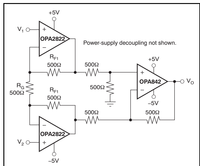
Figure 40. Wideband Three-Op Amp Differencing Amplifier
