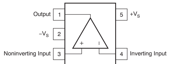
DRB PACKAGE SOT23-5 (TOP VIEW)
