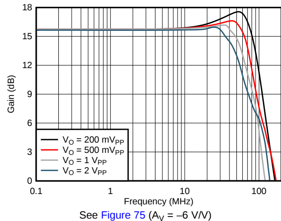
Figure 22. Inverting Large-Signal Bandwidth vs V_{OPP}
