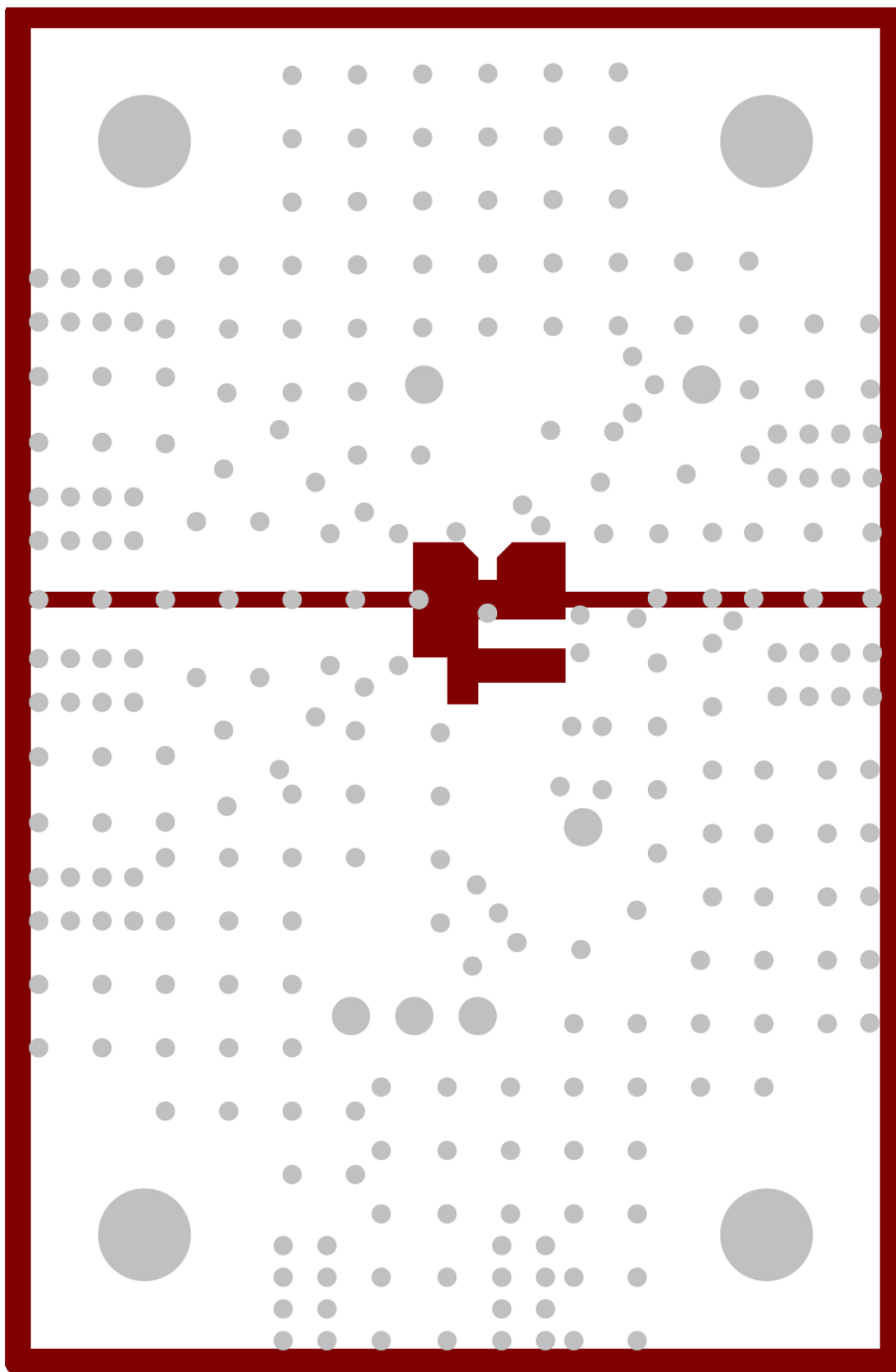
Figure 4. OPA837DBVEVM Layer 3
