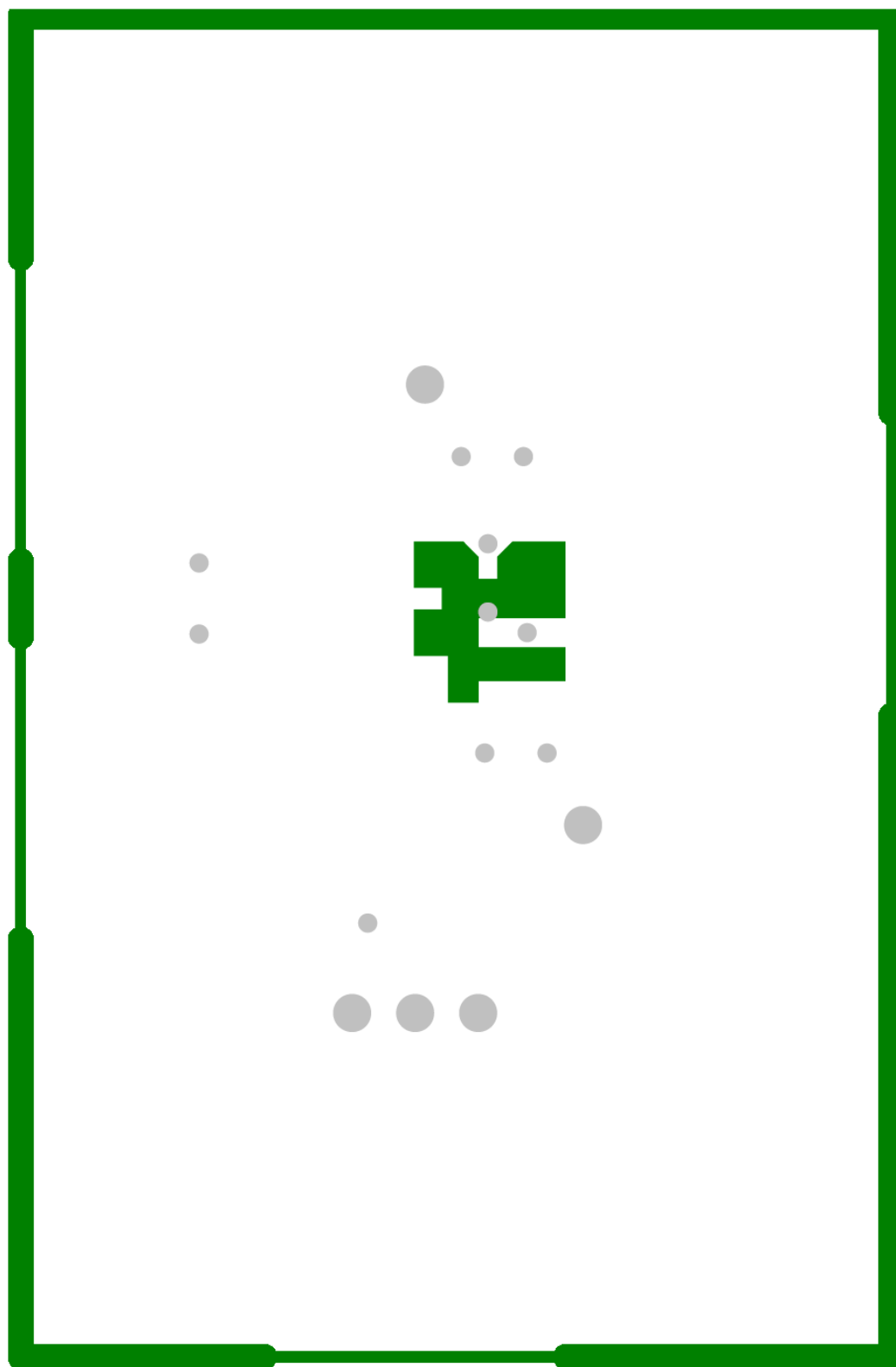
Figure 3. OPA837DBVEVM Layer 2
