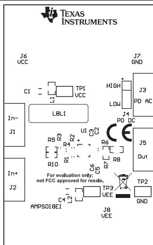
Figure 2. Top Overlay
