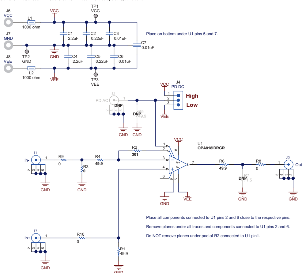
Figure 1. OPA818DRGEVM Schematic
