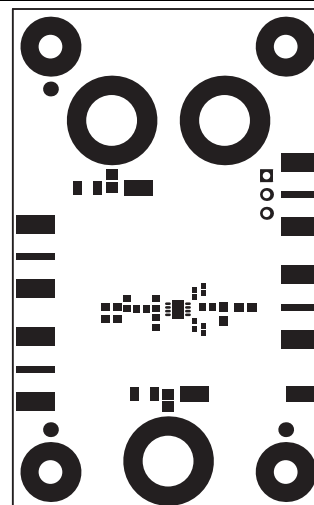
Figure 3. Top Solder
