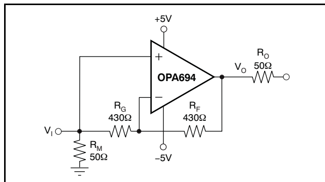
Figure 36. Improve Unity Gain Buffer
