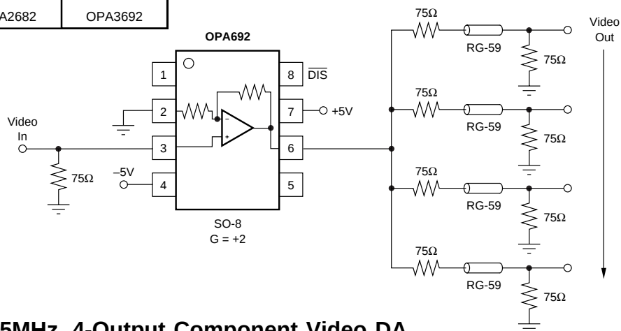
225MHz, 4-Output Component Video DA
