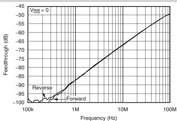
Figure 6. Disable Feedthrough vs Frequency
