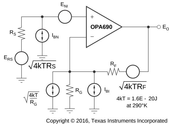
Figure 41. Op Amp Noise Analysis Model
