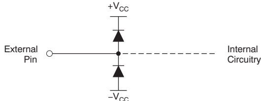
Figure 51. Internal ESD Protection
