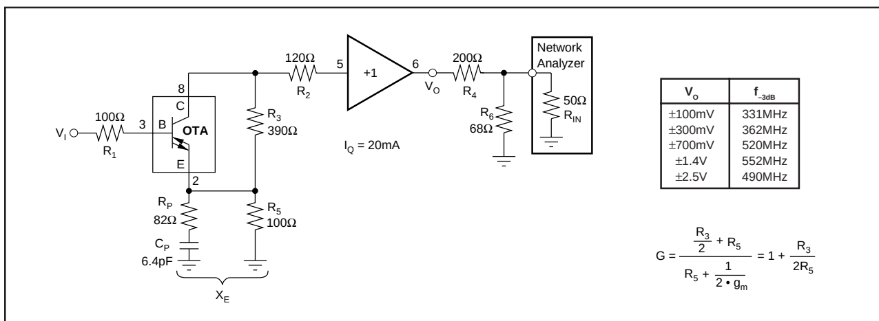
FIGURE 23. Direct-Feedback Amplifier.
