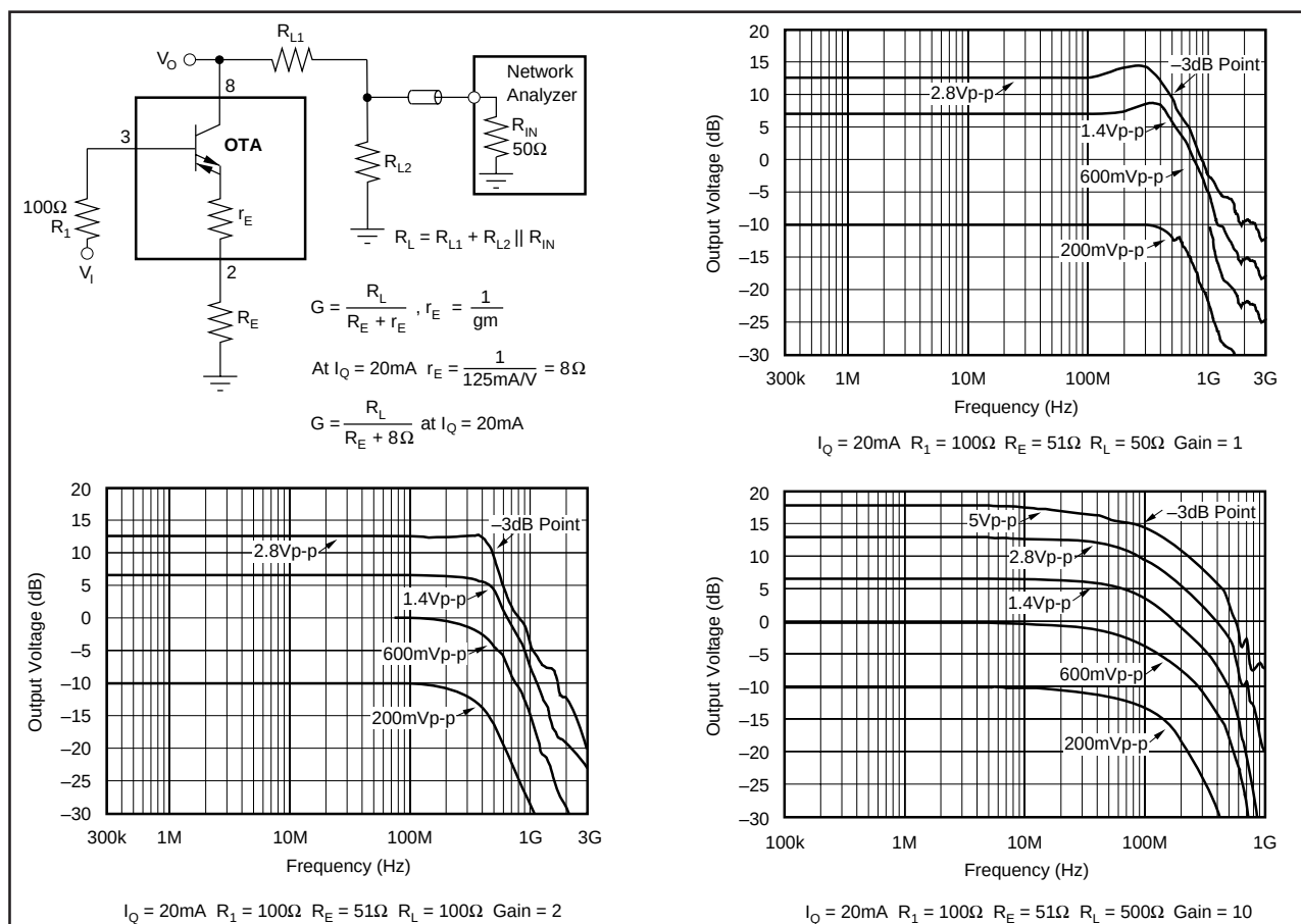
FIGURE 8. Common-E Amplifier Performance.
