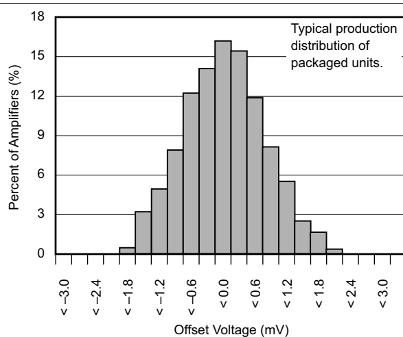
Figure 16. Offset Voltage Production Distribution
