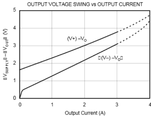
Figure 13. Output Voltage Swing vs Output Current
