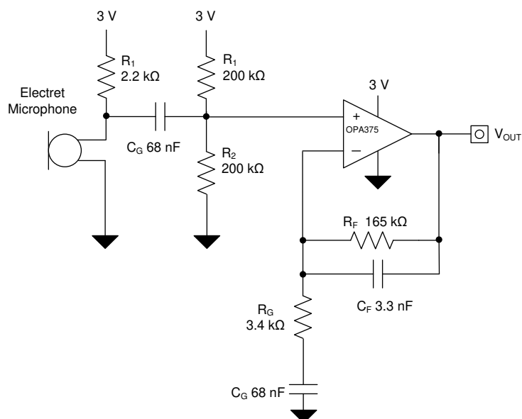
Figure 85. Microphone Preamplifier
