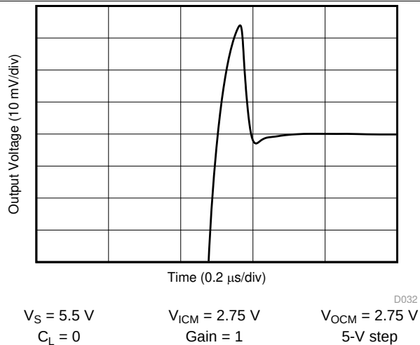
Figure 33. Large Signal Settling Time (Positive)
