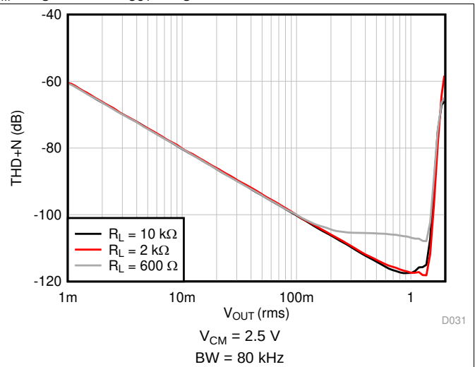
Figure 70. THD + N vs Amplitude
