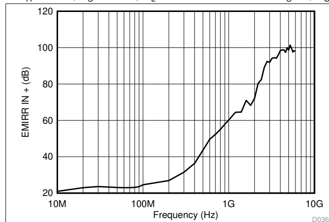
Figure 37. Electromagnetic Interference Rejection Ratio Referred to Noninverting Input (EMIRR+) vs Frequency
