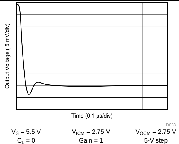
Figure 34. Large Signal Settling Time (Negative)
