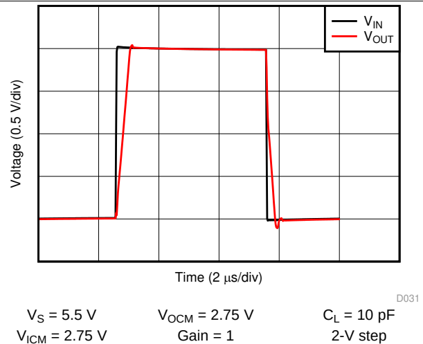
Figure 32. Large Signal Step Response
