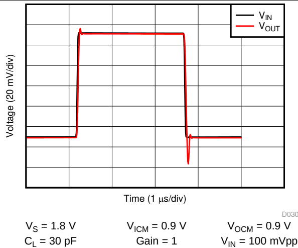
Figure 31. Small-Signal Step Response
