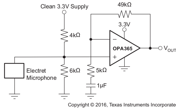
Figure 27. Microphone Preamplifier
