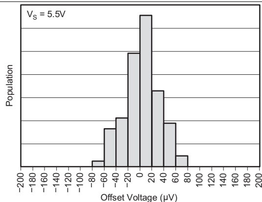
Figure 3. Offset Voltage Production Distribution
