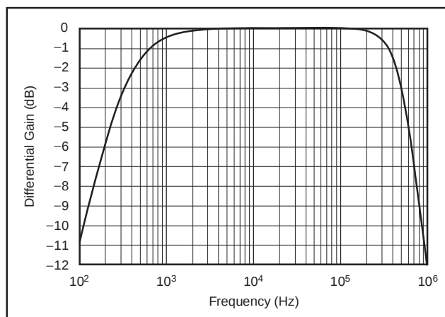
Figure 80. 5MHz, 2nd-Order, Butterworth Low-Pass Filter
