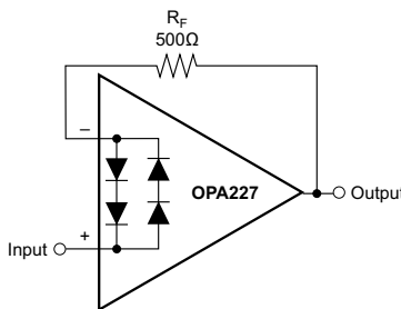
Figure 37. Pulsed Operation
