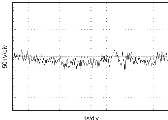
Figure 7. Input Noise Voltage vs Time
