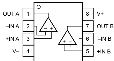
Pin Functions — SOT-23 (5), SOIC (8), and VSSOP (8) Packages
