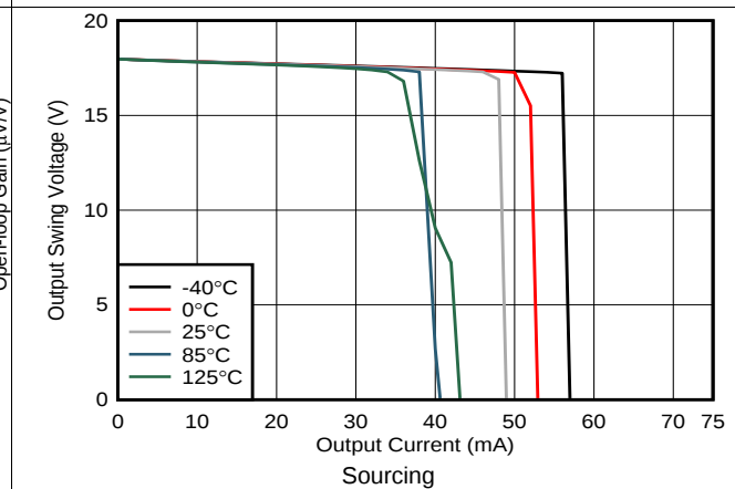
Figure 46. Output Voltage vs Output Current
