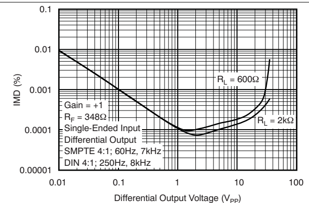
Figure 6. Intermodulation Distortion vs Output Voltage
