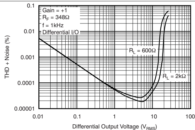
Figure 3. THD + Noise vs Output Voltage
