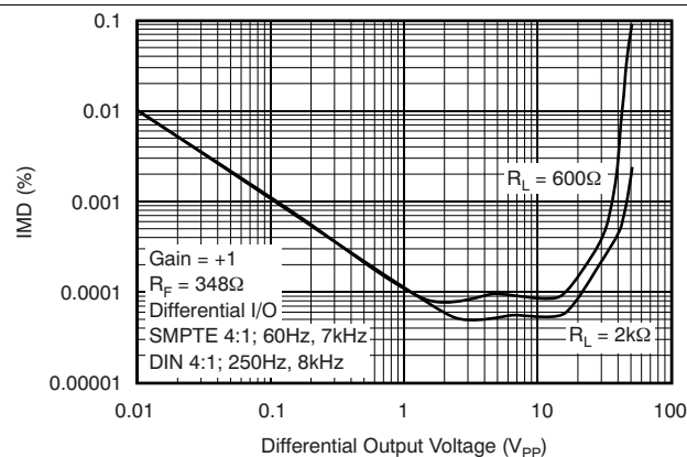
Figure 5. Intermodulation Distortion vs Output Voltage
