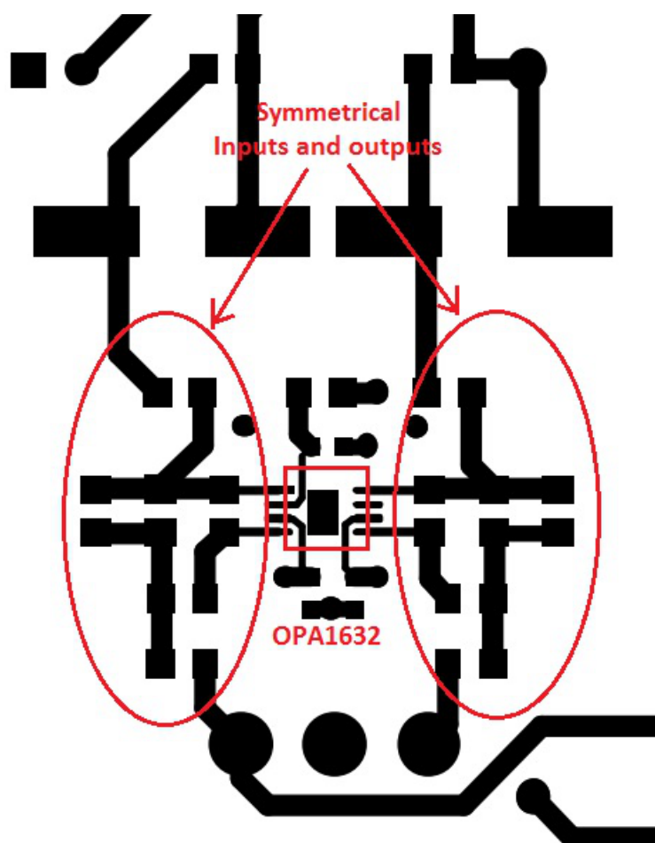
Figure 20. Example Layout
