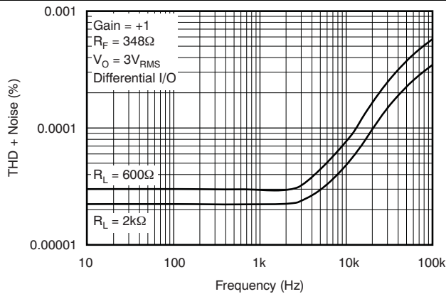
Figure 1. THD + Noise vs Frequency
