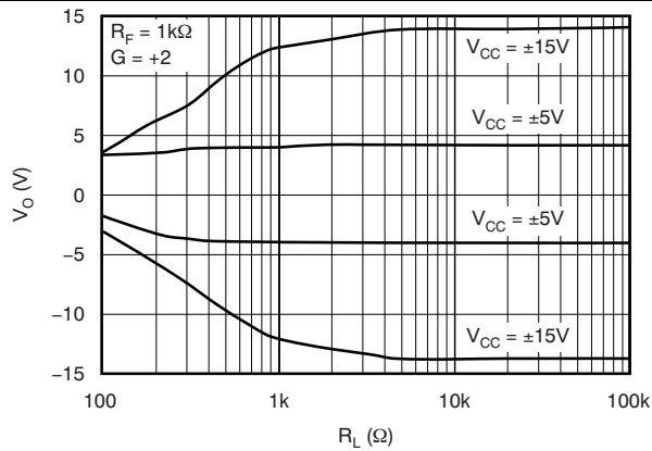
Figure 9. Output Voltage vs Differential Load Resistance
