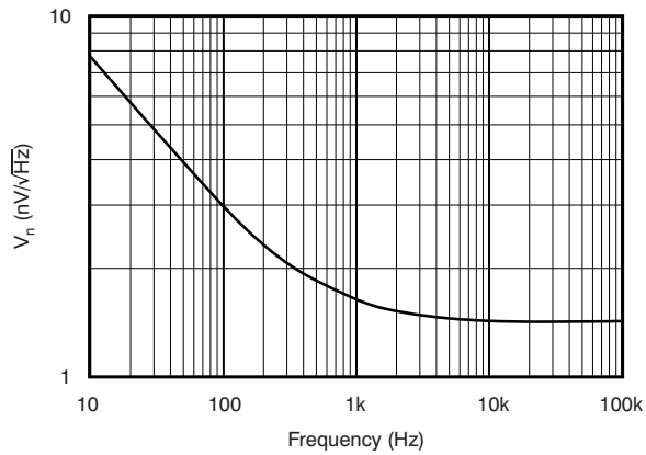
Figure 7. Voltage Noise vs Frequency
