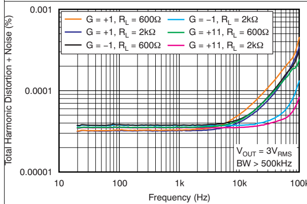
Figure 7. THD+N Ratio vs Frequency
