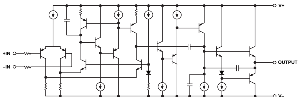
Figure 3. Simplified Schematic
