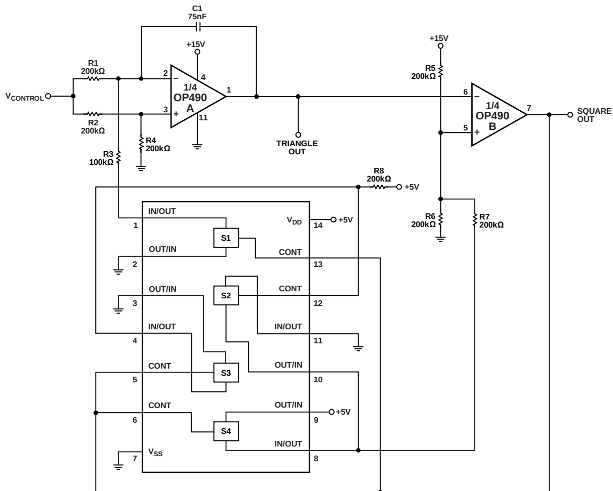
Figure 22. Micropower Voltage Controlled Oscillator
