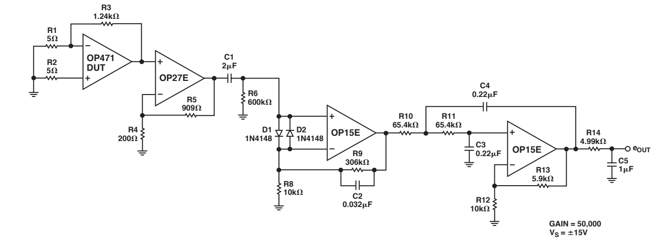
Figure 7. Peak-to-Peak Voltage Noise Test Circuit (0.1 Hz to 10 Hz)
