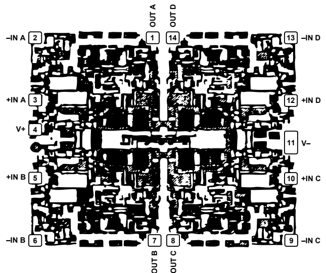
Figure 5. 0.111 Inch x 0.100 Inch DIE Size, 11,100 sq. mils, Substrate Connected to V+, 165 Transistors
