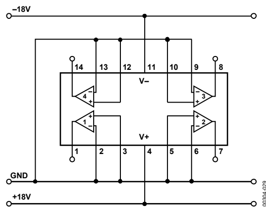
Figure 29. Burn-In Circuit
