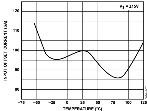
Figure 7. Input Offset Current vs. Temperature
