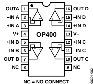
Figure 2. 16-Lead Standard Small Outline Package [SOIC_W]
