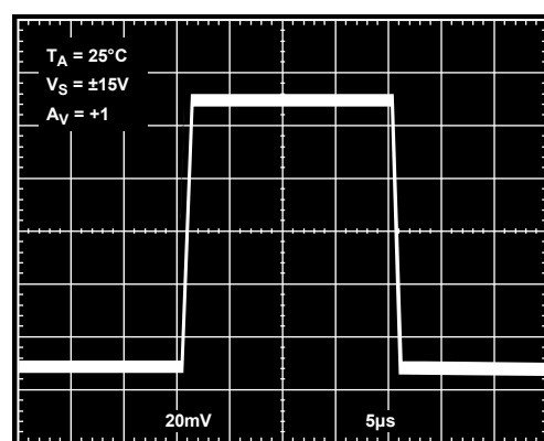
Figure 26. Small Signal Transient Response
