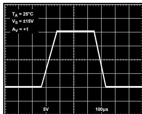
Figure 25. Large Signal Transient Response
