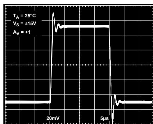
Figure 27. Small Signal Transient Response, C_{LOAD} = 1\text{ nF}
