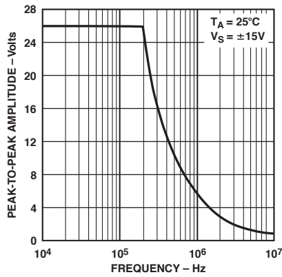
TPC 20. Maximum Output Swing vs. Frequency
