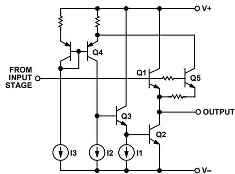
Figure 25. OP193/OP293 Equivalent Output Circuit
