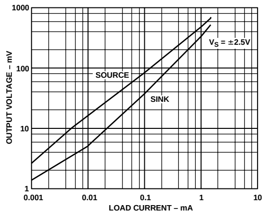
TPC 11. Output Voltage to Supply Rail vs. Load Current
