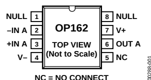
Figure 1. 8-Lead Narrow-Body SOIC (S Suffix)
