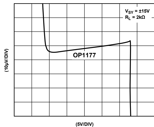
Figure 51. Gain Linearity
