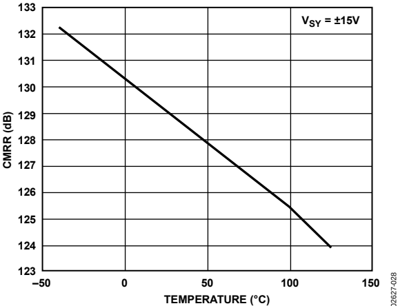
Figure 28. CMRR vs. Temperature
