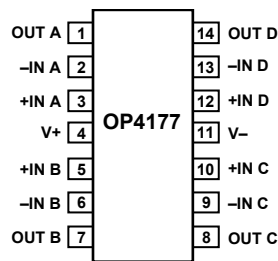
Figure 5. 14-Lead SOIC_N (R Suffix)
