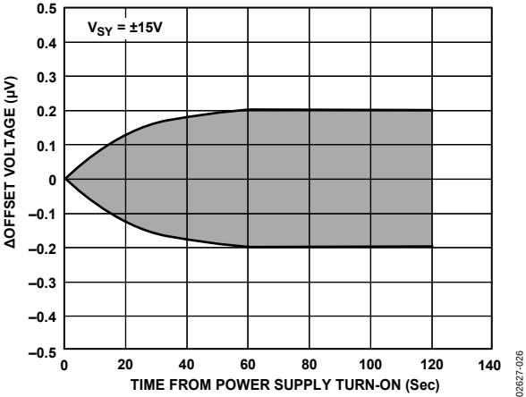
Figure 26. Warm-Up Drift
