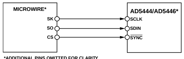
Figure 52. MICROWIRE to AD5444/AD5446 Interface
