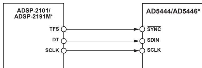
Figure 47. ADSP-2101/ADSP-2191M to AD5444/AD5446 Interface
