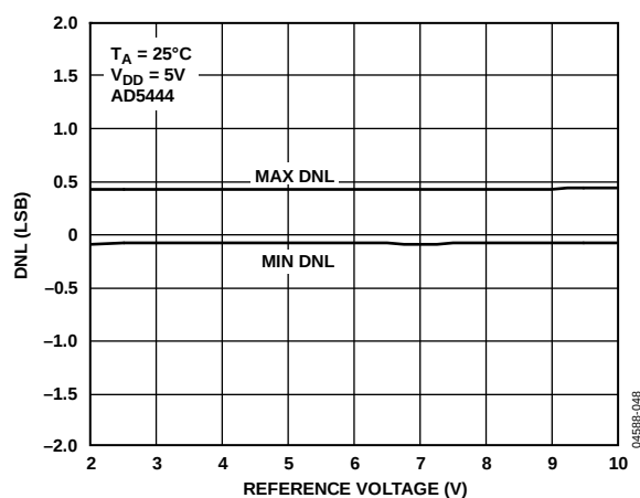
Figure 11. DNL vs. Reference Voltage
