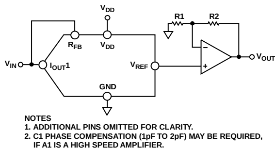
Figure 40. Single-Supply Voltage Switching Mode Operation
