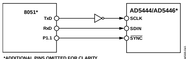
Figure 50. 80C51/80L51 to AD5444/AD5446 Interface
