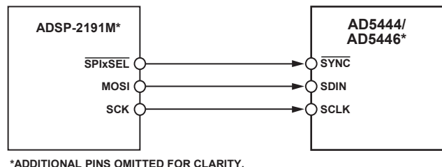
Figure 46. ADSP-2191M SPI to AD5444/AD5446 Interface
