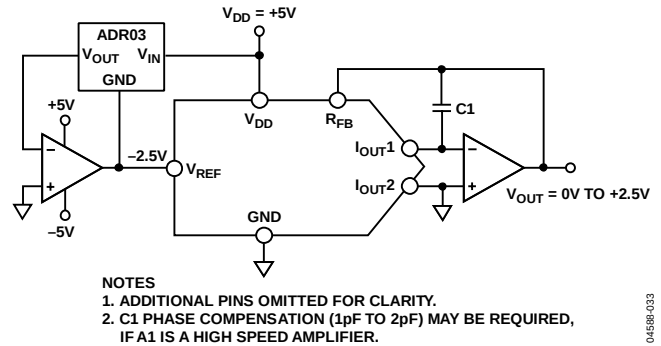
Figure 41. Positive Voltage Output with Minimum Components
