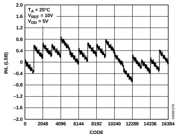
Figure 13. TUE vs. Code (14-Bit DAC)
