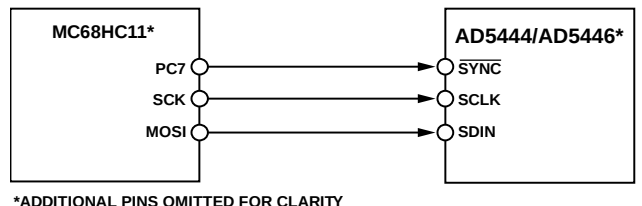
Figure 51. MC68HC11 to AD5444/AD5446 Interface
