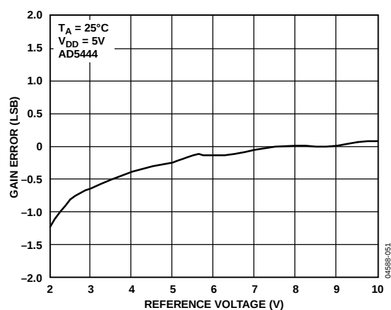
Figure 16. Gain Error vs. Reference Voltage
