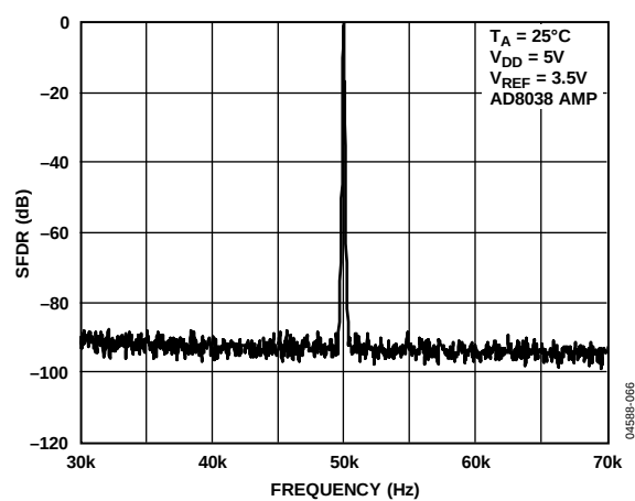
Figure 33. Narrow-Band SFDR, f_{OUT} = 50 kHz, Clock = 1 MHz
