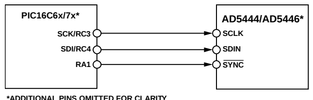
Figure 53. PIC16C6x/7x to AD5444/AD5446 Interface
