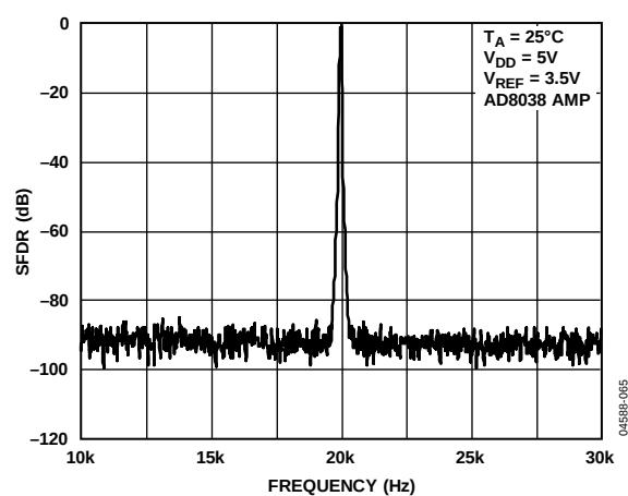
Figure 32. Narrow-Band SFDR, f_{OUT} = 20 kHz, Clock = 1 MHz
