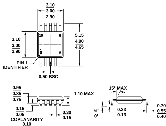
Figure 54. 10-Lead Mini Small Outline Package [MSOP] (RM-10)
