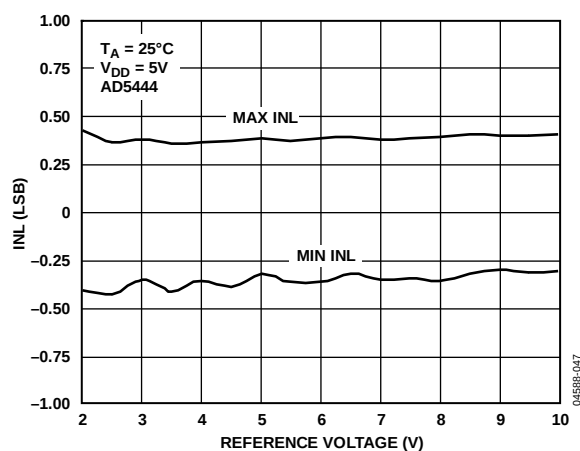
Figure 10. INL vs. Reference Voltage
