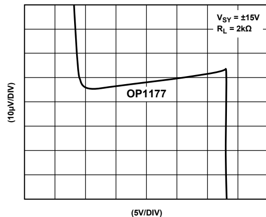
Figure 51. Gain Linearity
