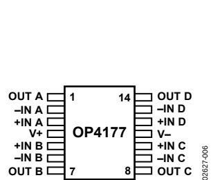
Figure 6. 14-Lead TSSOP (RU Suffix)
