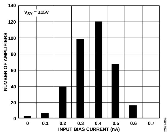
Figure 9. Input Bias Current Distribution
